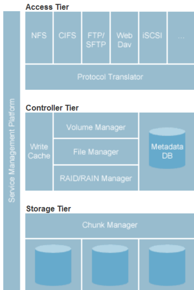
Native File System, System Architecture
